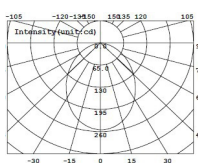
Difusor opal plano Flat opal diffuser
